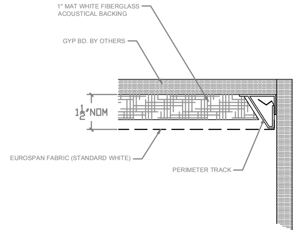
B EDGE AT WALL/SOFFIT 1.5GYP HALF SCALE
