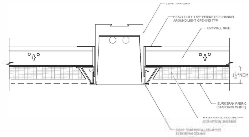
I TYPICAL @ LINEAR LIGHT TRIM FLANGE OVER EUROSPAN® (DRYWALL GRID) HALF SCALE
