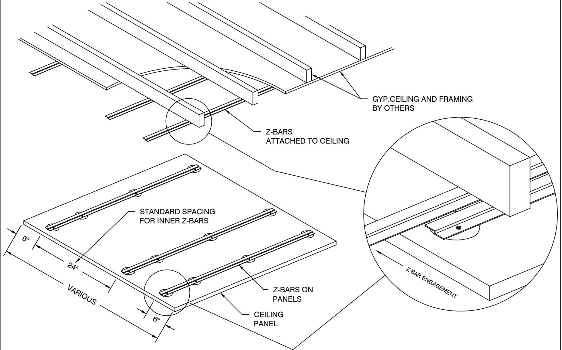
1 1.0 Z-BAR CEILING MOUNTING DETAIL (CONCEPTUAL DRAWING) SCALE: N.T.S.
