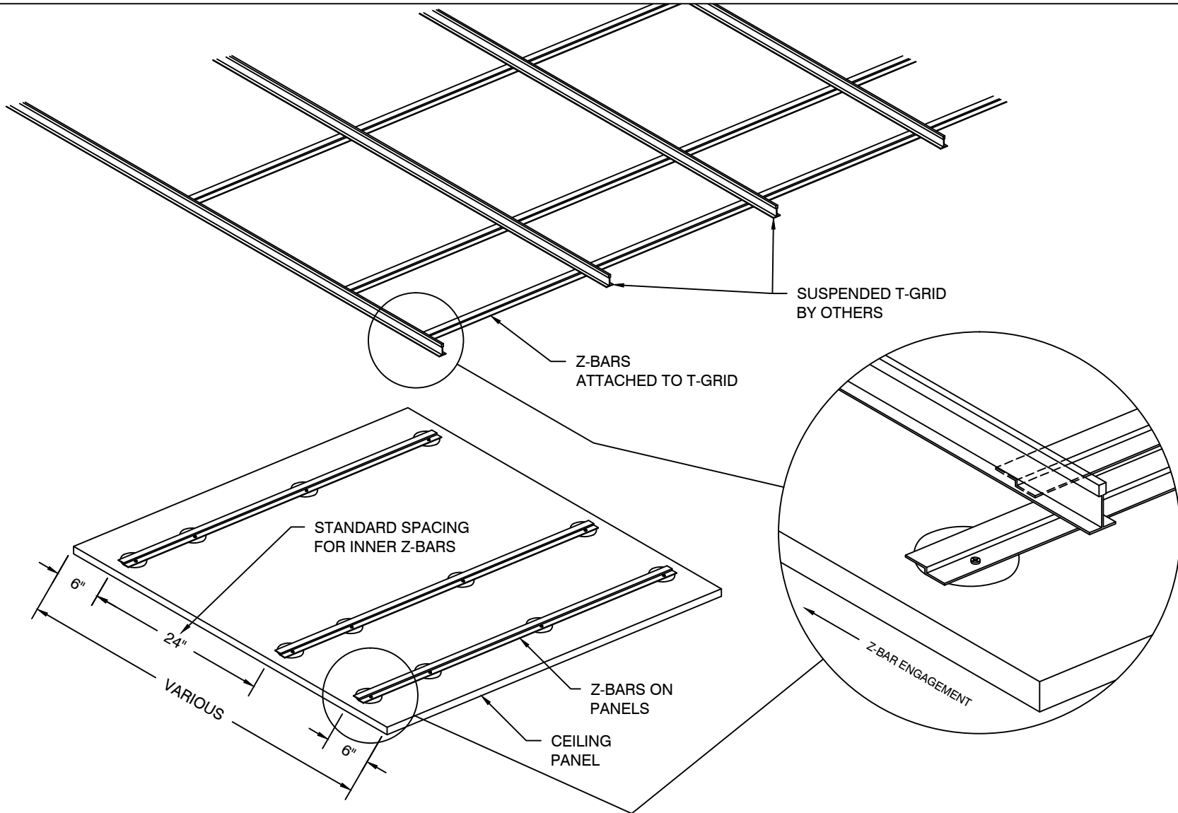
1 1.0 Z-BAR CEILING MOUNTING DETAIL (CONCEPTUAL DRAWING) SCALE: N.T.S.
