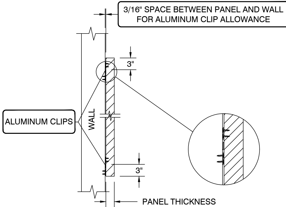
1 1.0 ACOUSTICAL PANEL MOUNTING DETAIL WITH ALUMINUM MOUNTING CLIPS SCALE: N.T.S.
