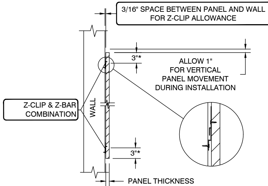
1 1.0 ACOUSTICAL PANEL MOUNTING DETAIL Z-CLIP WITH Z-BAR SCALE: N.T.S.
