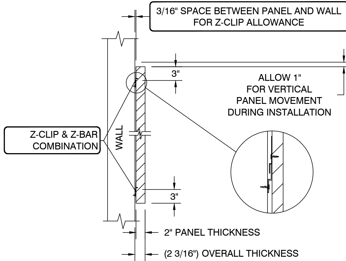
1 1.0 ACOUSTICAL PANEL MOUNTING DETAIL Z-CLIP WITH Z-BAR SCALE: N.T.S.
