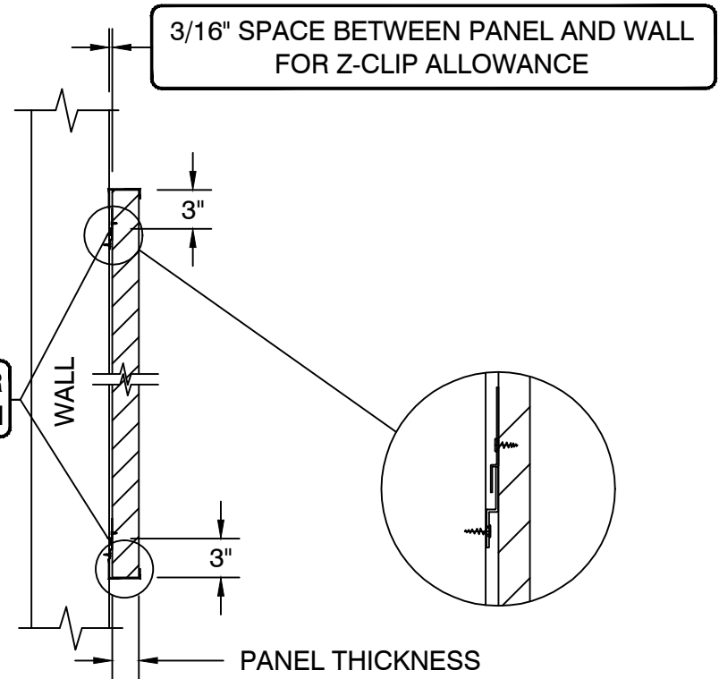
2 PANEL MOUNTING DETAIL Z-CLIP WITH Z-BARS SCALE: N.T.S.
